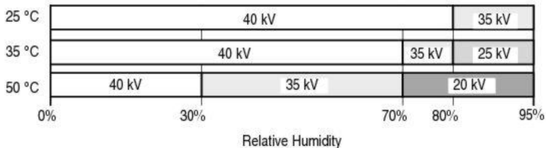
Figure 1-7: Humidity Derating Chart
