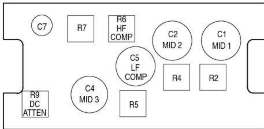
Figure 2-2: Adjustment Locations
